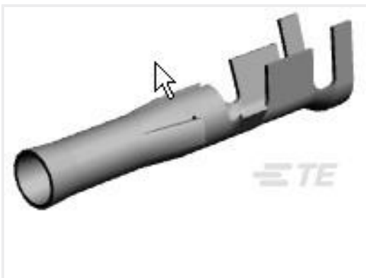
TE 产品编号770144-6 .093 CP&S SOC PTPPHBZ LP 20-14
