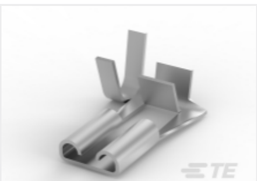
TE 产品编号1742718-1 250 FASTON,FLAG,REC.,16-12 AWG, TPBR
