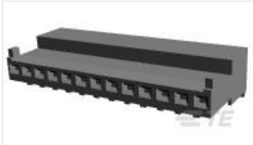
TE 产品编号4-643814-3 13P MTA100 CONN ASSY POL RIB
