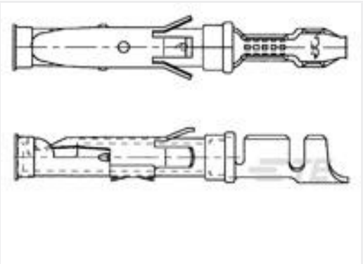
TE 产品编号1-163087-1 SPEC.PLATED
