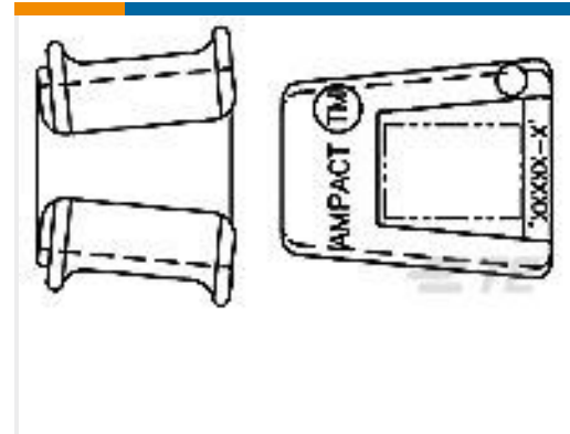
TE 产品编号602046-6 AMPACT Tap 266.8-3/0
