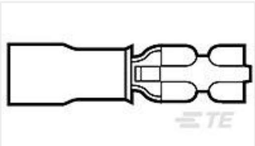
TE 产品编号640921-2 RECEPT,PIDG FASTON 22-18 110
