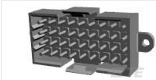
TE 产品编号207121-9 METRIMATE PIN HDR ASY,36P LF
