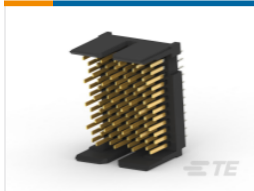
TE 产品编号2065798-3 Tin Man Header Assy 4x8Open
