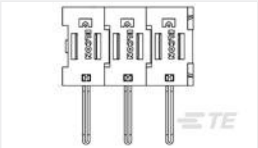
TE 产品编号6646911-1 CONN,PIN,RT<,SLDR,FLATPAQ
