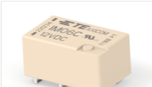
TE 产品编号3-1462039-4 IM06CJR=IM RELAY 140mW12V HDV
