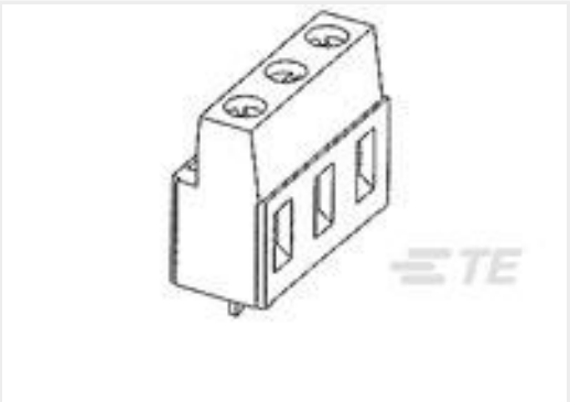
TE 产品编号282845-3 TERM-BLOK,PCB MNT,90DG,3P,7.62
