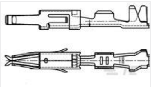
TE 产品编号962943-1 MT2 REC 1.6 Contact SRC Sn
