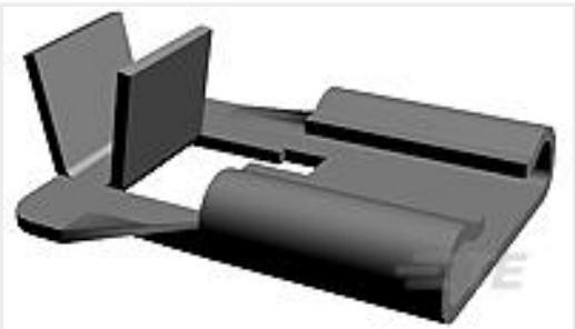
TE 产品编号63096-1 250 FASTON FLAG REC 18-14 AWG BR
