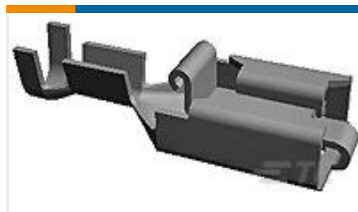
TE 产品编号927854-2 PL 250 REC TERMINAL 17-13 AWG PBR
