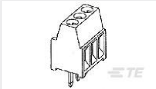
TE 产品编号1546215-4 TERMI-BLOK PCB MOUNT, 90 4P.
