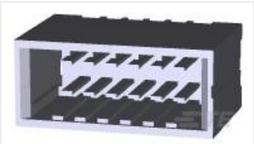
TE 产品编号178326-3 DYNAMIC DBL ROW HDR ASSY 12P V
