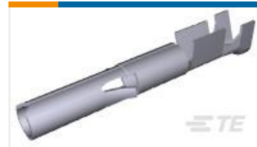
TE 产品编号350689-7 UMNL SOK 24-18 AUBR L/P
