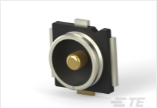
TE 产品编号2334884-1 UMCC Micro-Coax receptacle, Gen 4
