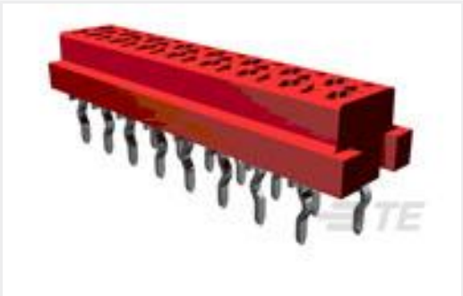
TE 产品编号8-215079-6 MICRO-MATCH FOB.16P
