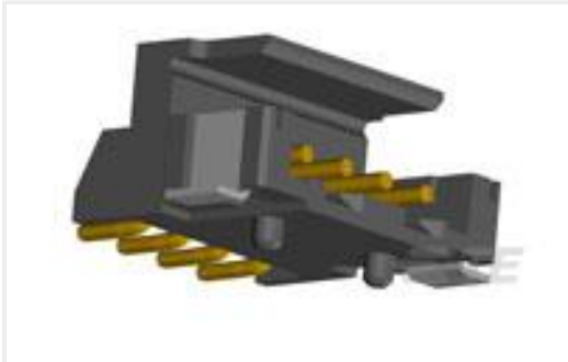
TE 产品编号3-292173-2 CT BOX HDR H SMT 2P O/TAPE NAT
