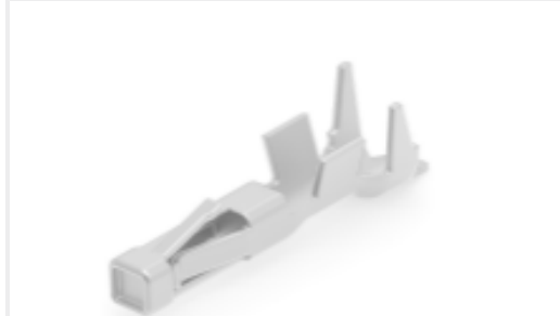
TE 产品编号1-2834067-2 SOCKET CONTACT,MINIATURE WATERPROOF CONN
