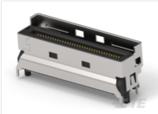
TE 产品编号1-2379397-6 MCIO INTERGRATED CONN, V/T,8X, SMT TYPE
