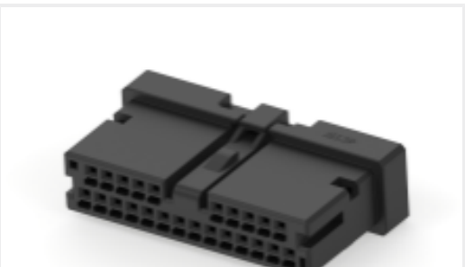
TE 产品编号2-2834627-4 MD REC HSG ASSY 24P X-KEY BLK HF BLK
