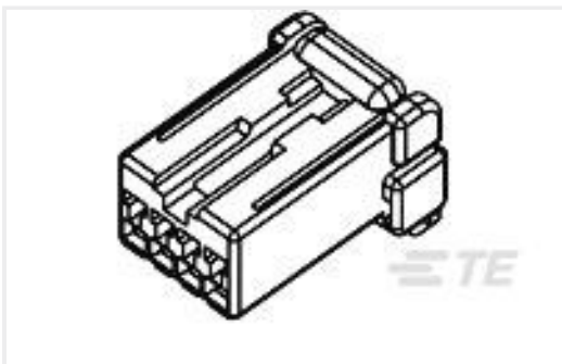
TE 产品编号175507-2 040 MULTI-LOCK I/O PLUG HSG 6P
