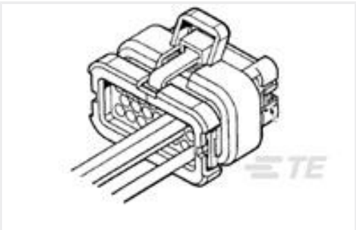
TE 产品编号776273-1 14POS, AMPSEAL, SOC HSG ASSY, SLD, COD 1
