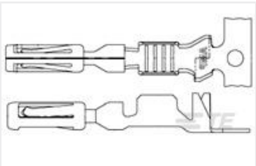
TE 产品编号770520-1 AMPSEAL, TERMINAL, TIN PLATE, 16-20AWG WIRE
