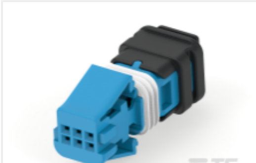
TE 产品编号3-2112594-3 6POS,NANOMQS,REC HSG ASSY, SLD,COD C
