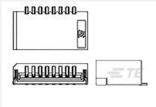
TE 产品编号84981-4 1MM FFC SMT H ASSY 4P EMBOSS
