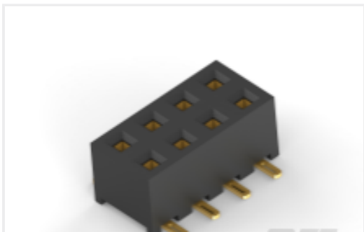
TE 产品编号2271597-8 AMPMODU, REC HDR,DR, 2.0PITCH, SMT, 8P
