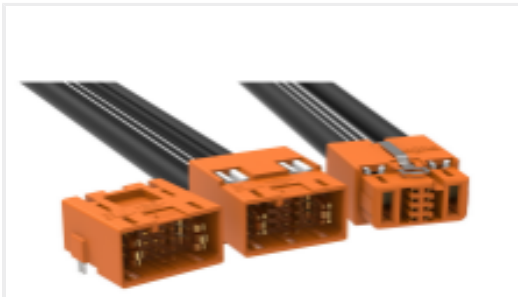
TE 产品编号2332798-8 UMP, CONNKIT, PWRSGNL, PANEL, 8AWG
