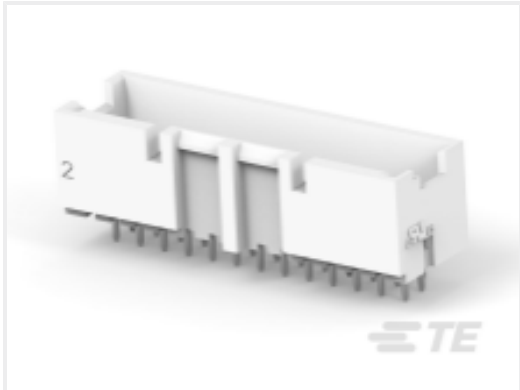
TE 产品编号2-2324245-6 ASSY,HDR,VERT,GWT,BOSSED,DUAL ROW, EP2.5
