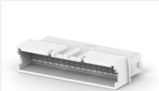
TE 产品编号 3-2324201-4 HSG,REC,FREE-HANGING,GWT, DUALROW,EP2.5
