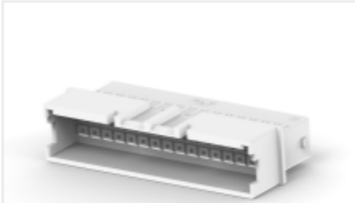
TE 产品编号 3-2324201-2 HSG,REC,FREE-HANGING,GWT, DUALROW,EP2.5
