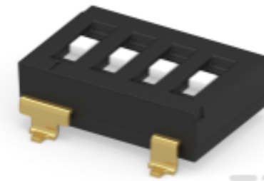
TE 产品编号 2-2319747-6 TRI-STATE DIP 4P G RECESS SEAL T&R
