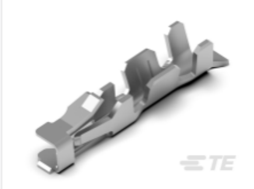
TE 产品编号2-2316113-3 2MM,REC,CNT,CRIMP,24-28AWG,TIN, LP
