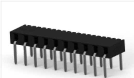
TE 产品编号1-2314938-0 10P,2MM,B-B,REC,SRHZ,2.8,0.76AU,TR
