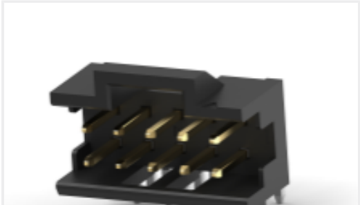
TE 产品编号1-2823411-2 12P,2MM,PL HDR,DRRT,2.8,0.76AU,TB
