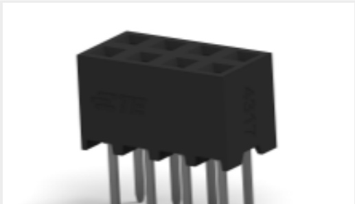
TE 产品编号2314824-8 8P,2MM,B-B,REC,DRVVT,2.7,0.1AU,TB, W/CAP
