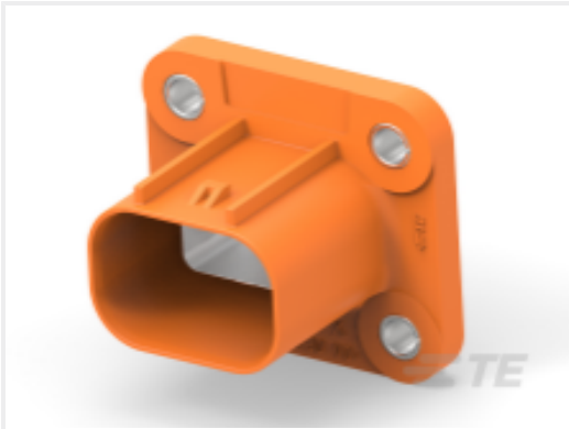
TE 产品编号2310541-1 SPLIT HEADER ASSY, KEY A, HVA280, V0
