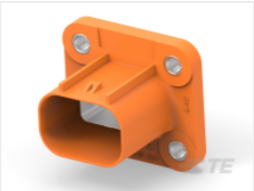
TE 产品编号2310541-2 SPLIT HEADER ASSY, KEY B, HVA280, V0
