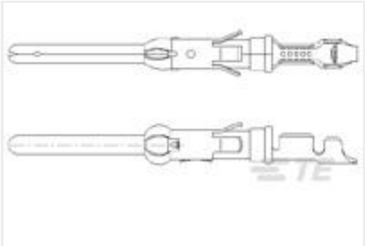
TE 产品编号163081-7 .062 DIA PIN ASSY 3+
