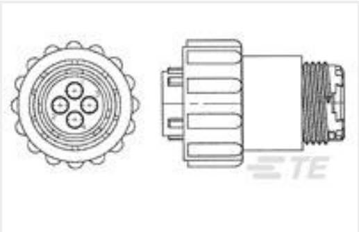
TE 产品编号796188-1 SLD CPC PLUG ASSY,23-24,STD SX
