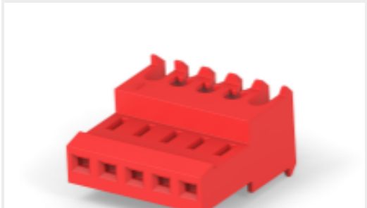
TE 产品编号CAT-104MTA-NGPNR Nylon Gold Plated Receptacle: 2.54 mm, no Mating Alignment
