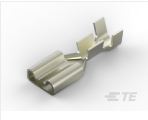
TE 产品编号2238196-3 FASTON 250 STD REC STR 18-14TPBR
