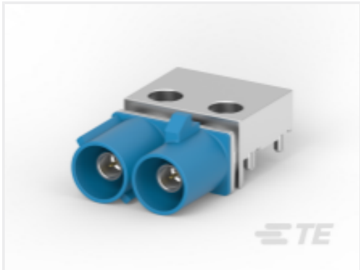
TE 产品编号5-2287923-3 FAKRA, 2 POS, EXT-EDGE, ASS'Y 12 O'CLOCK
