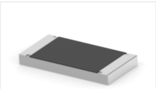
TE 产品编号2-2176350-8 CRGCQ 2512 33K 5%
