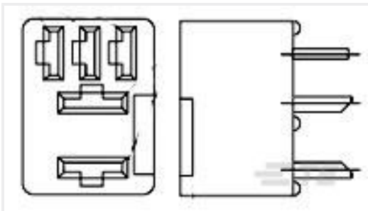
TE 产品编号1393310-2 VCFM-1000=FROM SEC
