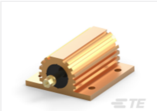
TE 产品编号5-2176731-4 HSC100S 1K5 5% Screw Terminal
