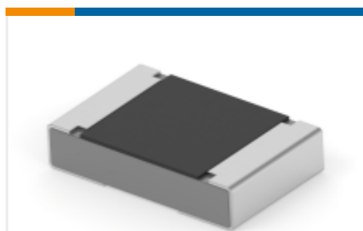
TE 产品编号4-2176482-3 RA73F 2A 140R 0.1% 5K RL
