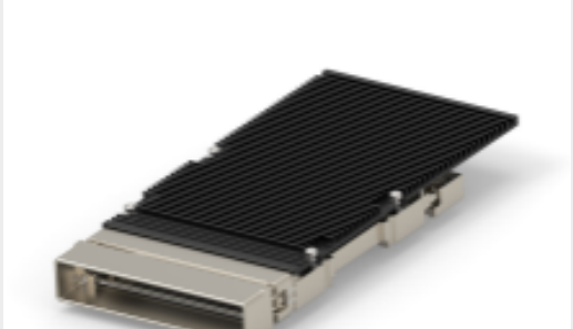
TE 产品编号2300837-1 Hardware Kit, CFP, 5mm Heatsink
