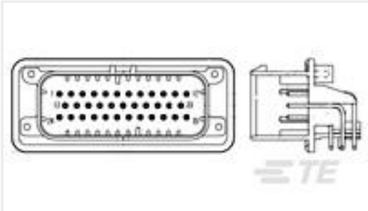
TE 产品编号776163-1 35POS,PIN DIA 1.3,HDR ASSY,90DEG, COD 1
