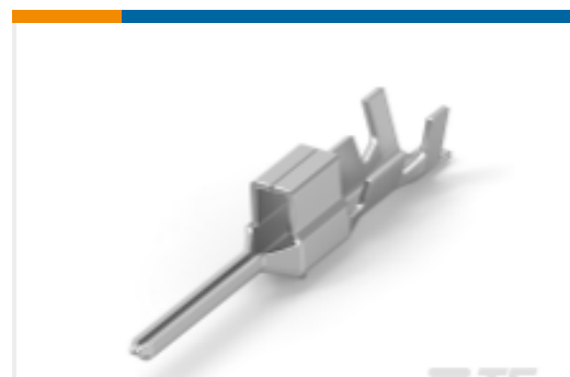
TE 产品编号2232575-1 2.5 SIGNAL D/LOCK TAB CONT. M
