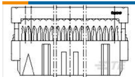
TE 零件编号5-826632-0 AMPMODU II PIN HEADER 50P
