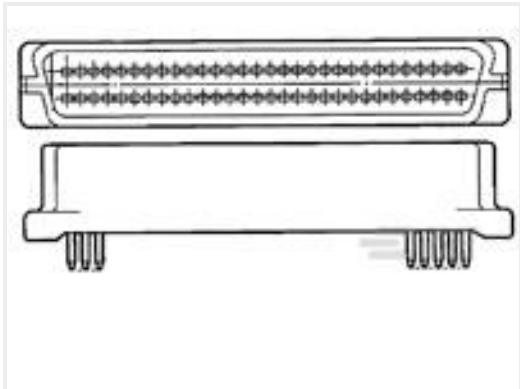
TE 产品编号5173280-3 AMPLIMITE.050 CAP ASS'Y (V) 50
