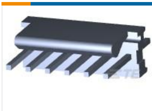
TE 产品编号641215-6 06P MTA100 HDR ASSY FL/ST 30AU
