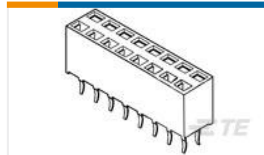
TE 产品编号2-215309-8 2X28P HV100 REC CON. TE, 8.5MM
