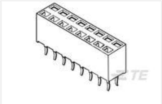
TE 产品编号215307-9 2X9P HV100 REC CON. TE, 7.0MM
